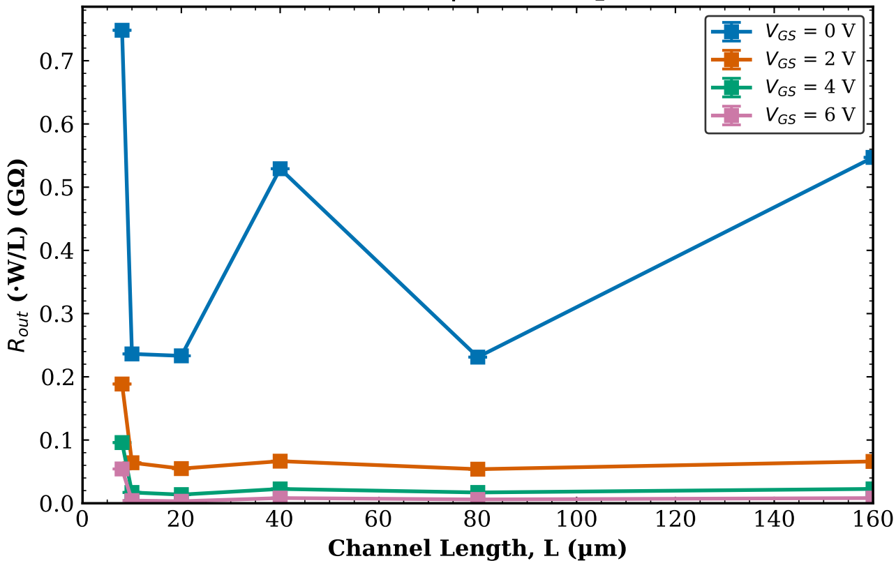
TFT1 Transistor 1 R_{out} vs L | W = 10\text{ }\mu\text{m}
